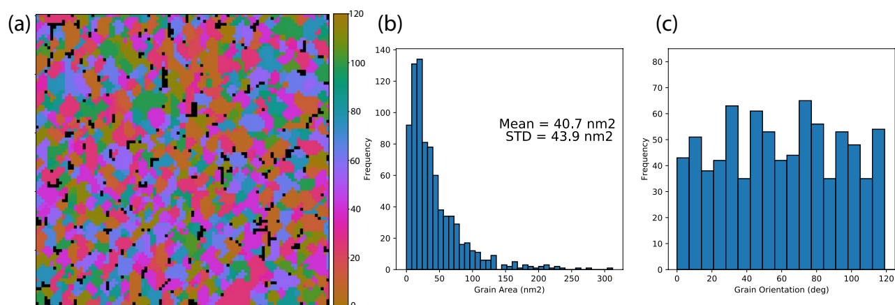
Figure 7. Results of MVA grain size/orientation analysis for polycrystalline \text{WS}_2 . The image in (a) shows the spatial distribution of distinct crystalline grains, with the color scale indicating the crystallographic orientation. The black regions are voids where no crystallographic component has appreciable value. The histogram in (b) shows the distribution of grain areas, peaking at 10 \text{nm}^2 , and dropping to near zero at 150 \text{nm}^2 . The grain orientation angle distribution is shown in (c). The orientation is defined by the angle of the most intense peak of the k-space component, modulo 120 degrees (due to the three-fold symmetry of the underlying 1H lattice). The distribution is approximately flat, indicating no preferred grain orientation.
